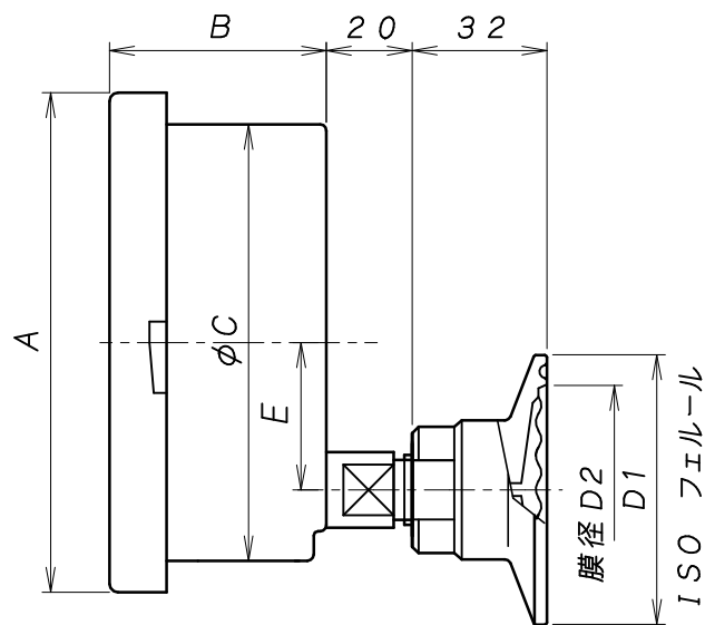
ISO CLAMP FITTING FERRULE
